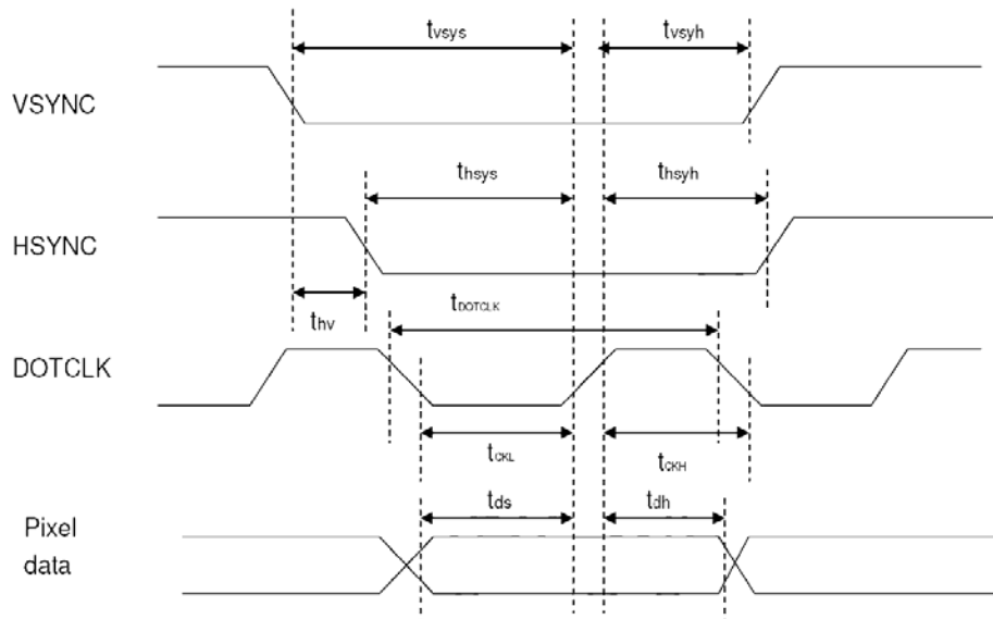
Figure 14. 1 Pixel Timing
