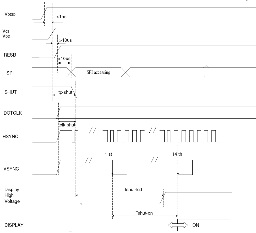
Figure 14. 10 Power Up Sequence
