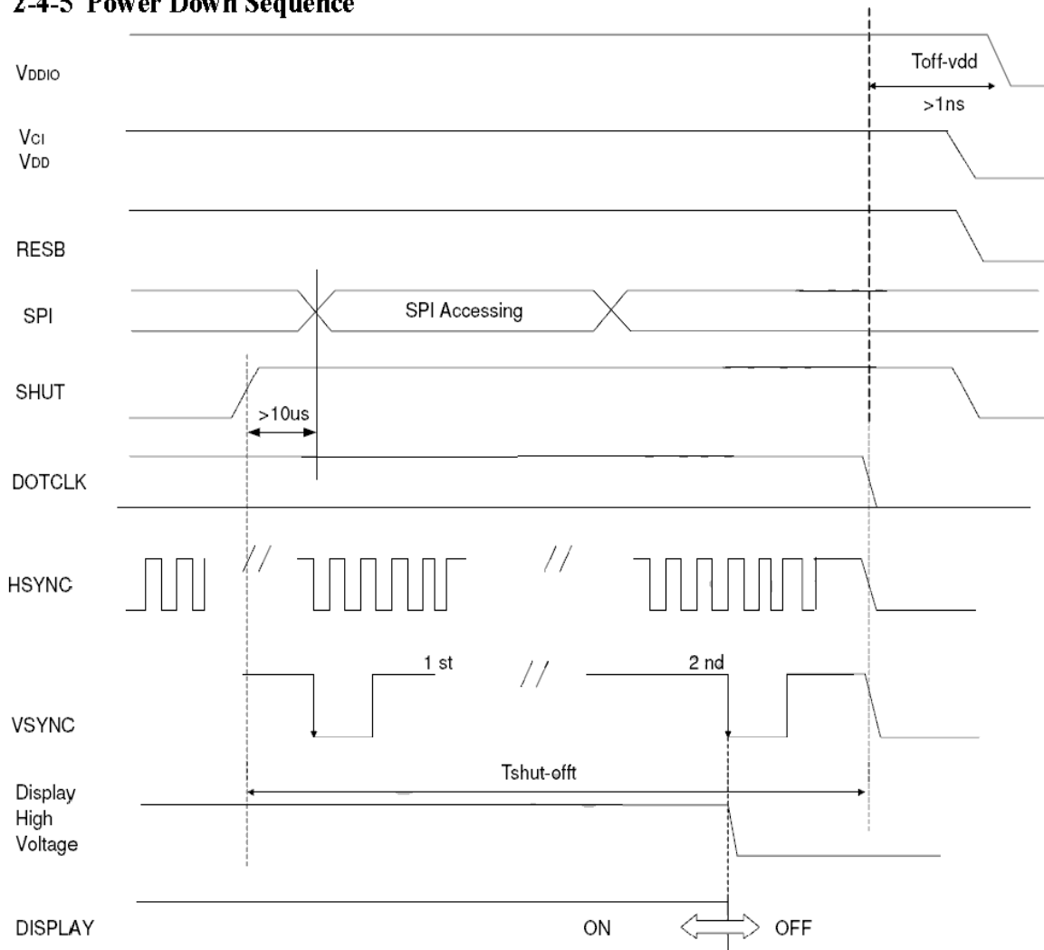
Figure 14. 11 Power Down Sequence
